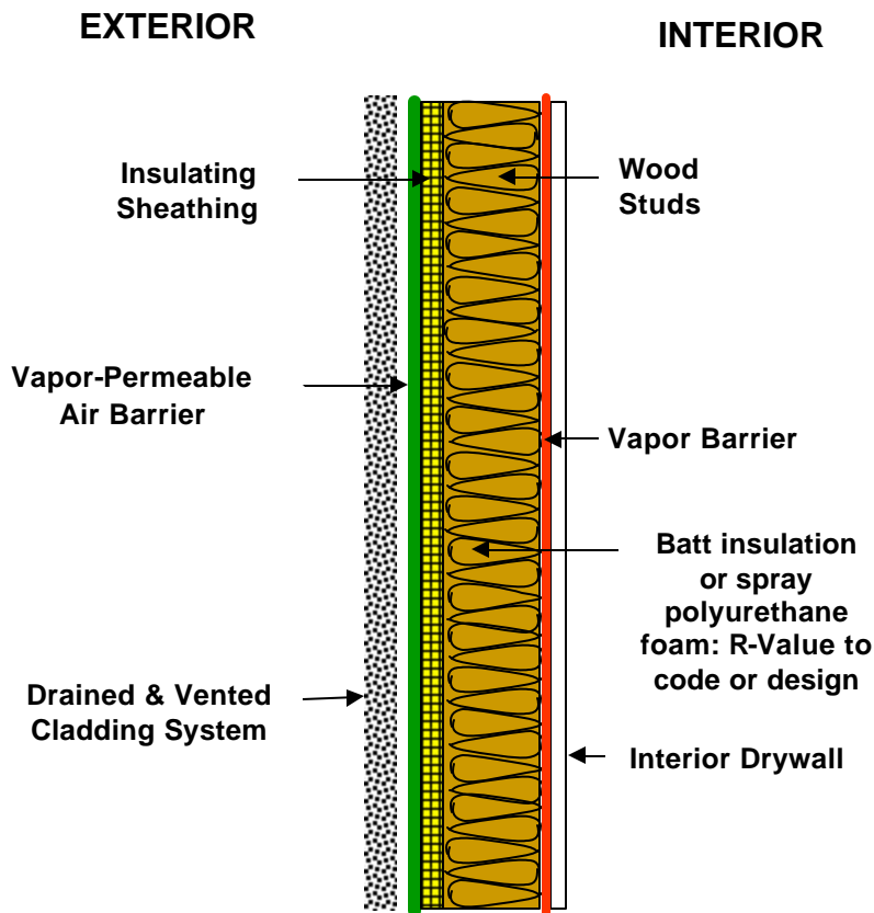
Figure 5: Sheathing over Stud Wall System with Vapor-Permeable Air Barrier
