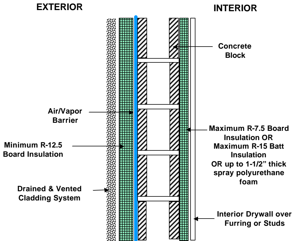
Figure 4: Mass Wall System with Air/Vapor Barrier for Zones 7 & 8
