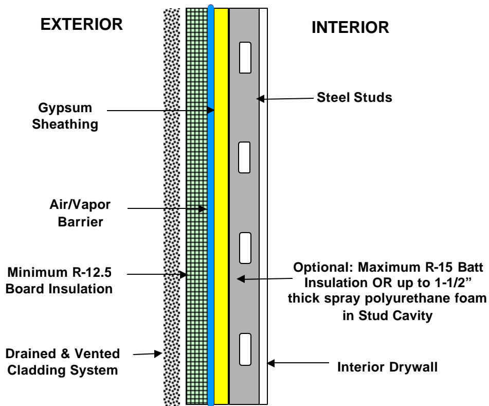
Figure 3: Steel Stud Wall System with Air/Vapor Barrier for Zones 7 & 8
